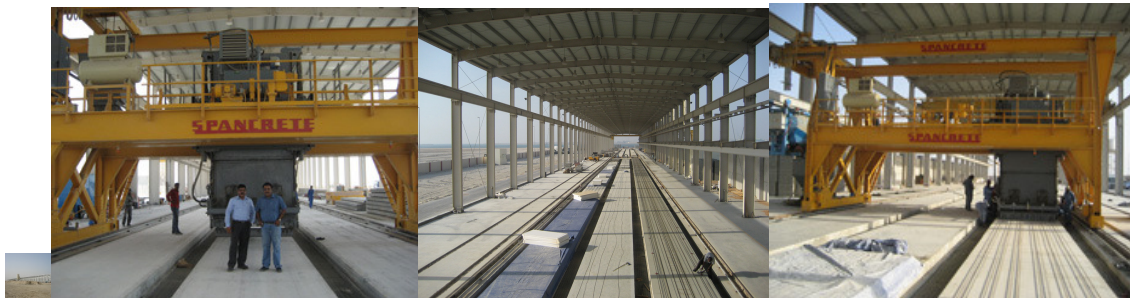
Hi-Tech's new Spancrete GT-240 system operating in their new production facility located in Abu Dhabi, UAE.
